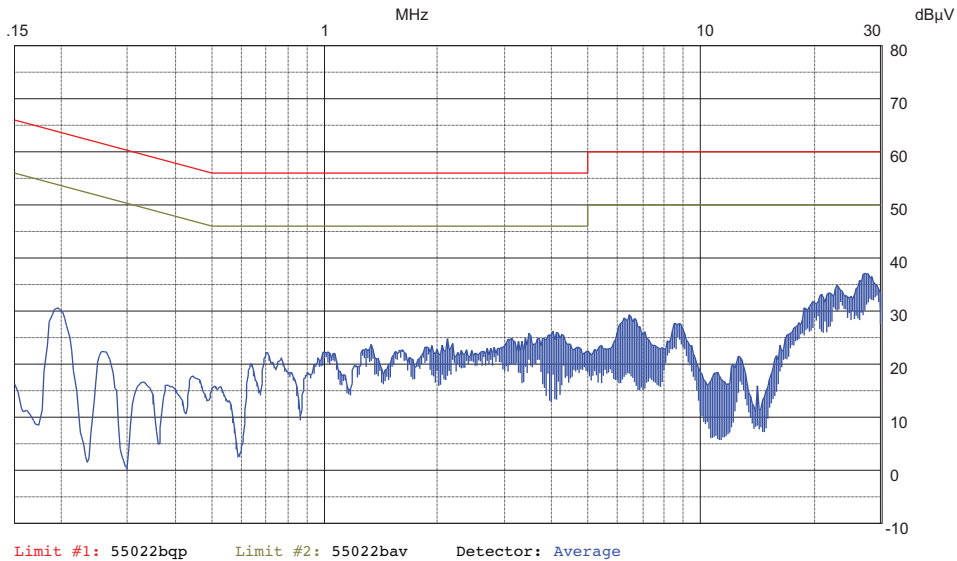
Figure 11 Typical conducted noise plot
