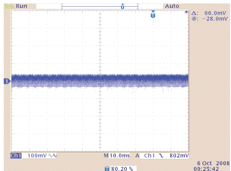
Figure 5 ECS100US12 (100 W) 66 mV pk-pk ripple. 20 MHz BW
