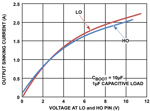
FIGURE 13. PEAK PULL-DOWN CURRENT vs OUTPUT VOLTAGE
