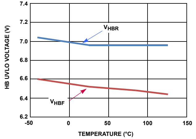
FIGURE 16. VHB UNDERVOLTAGE LOCKOUT THRESHOLD vs TEMPERATURE
