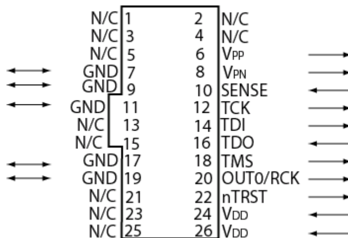
Figure 153 · 26-pin Connector for FlashPro Lite
