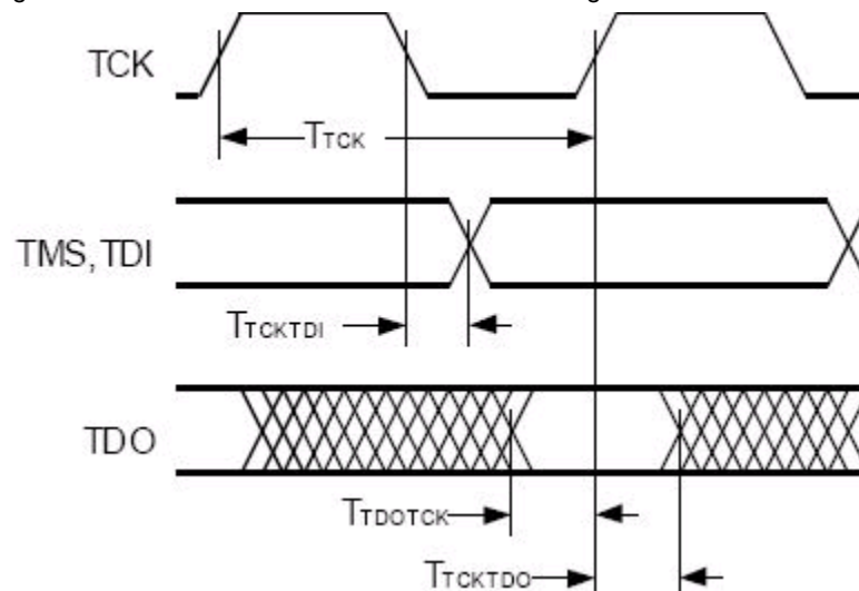
Figure 155 · JTAG Switching Characteristics
