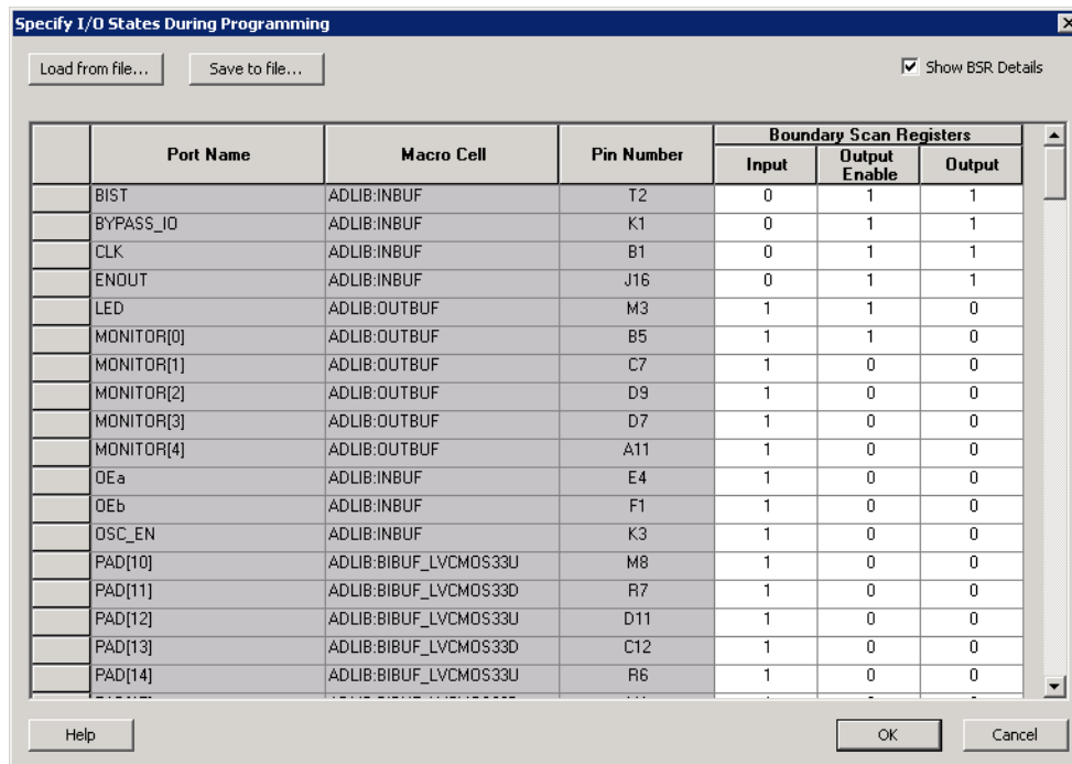
Figure 144 · Boundary Scan Registers
