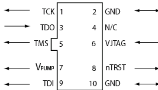
Figure 152 · FlashPro3 10-Pin Connector
