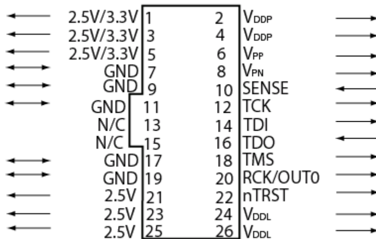
Figure 154 · 26-pin connections for FlashPro
