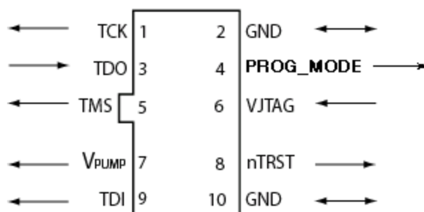
Figure 151 · FlashPro4 10-Pin Connector
