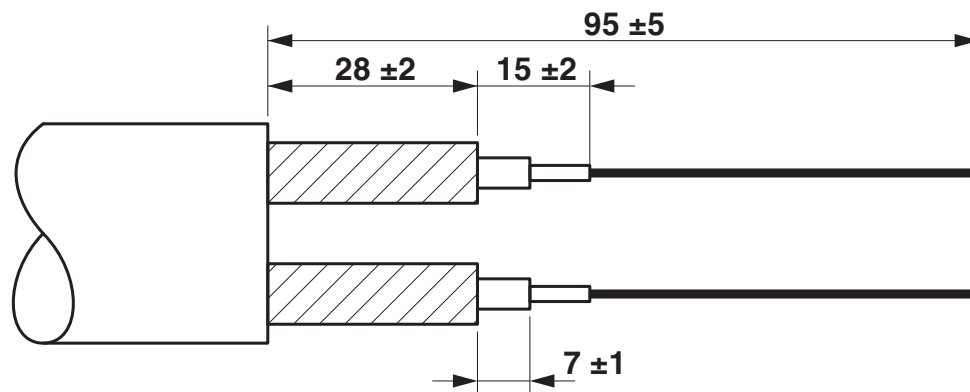
Dimensional drawing
