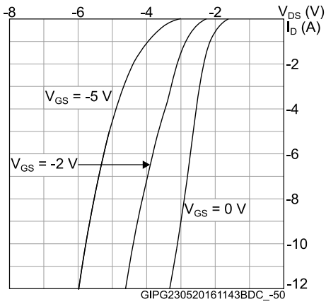
Figure 16: Body diode characteristics ( T_J = -50^\circ C )
