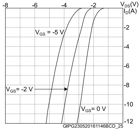
Figure 17: Body diode characteristics ( T_J = 25^\circ C )
