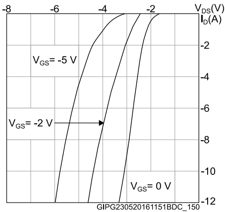
Figure 18: Body diode characteristics ( T_J = 150^\circ C )
