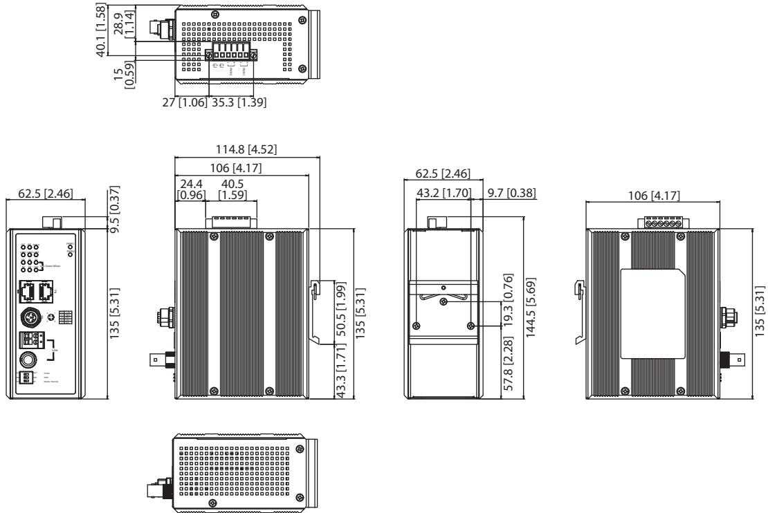
Panel Cut-out Dimensions: 62.5 x 135 x 106 mm (2.46" x 5.32" x 4.17")
