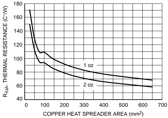
Figure 21. R θJA vs. Copper Spreader Area, SOT-223
