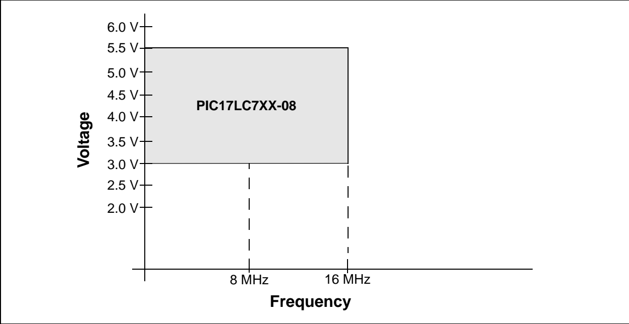
FIGURE 20-3: PIC17LC7XX-08 VOLTAGE-FREQUENCY GRAPH
